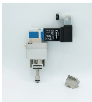
Speed-Coat® module (left) and Rhythm Elastic nozzle (right)
